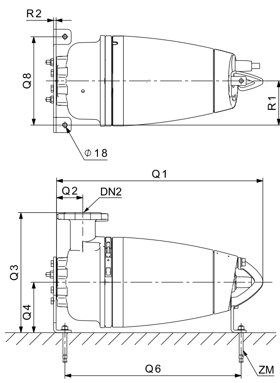
Рис. 10 SEV Dry horizontal installation
