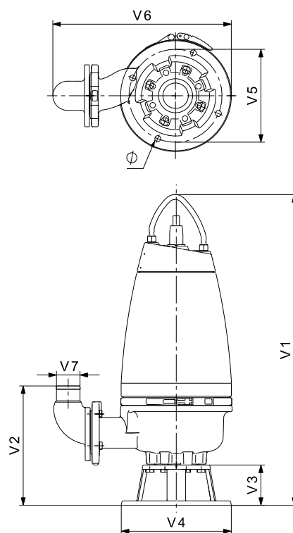
Рис. 6 SEV Free-standing submerged pump on ring stand
