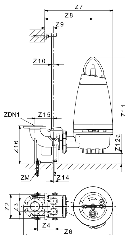
Рис. 8 SEV submerged pump on auto-coupling
