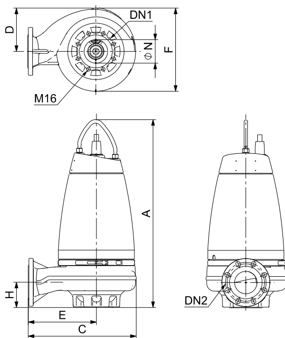
Рис. 2 SE1 pump without accessories
