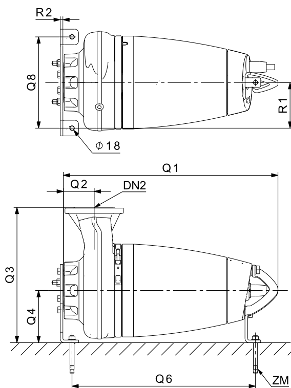
Рис. 9 SE1 Dry horizontal installation
