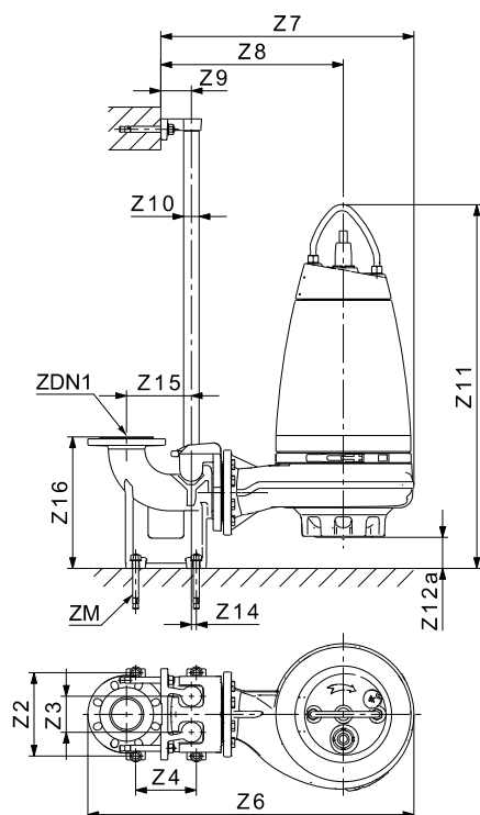
Рис. 7 SE1 submerged pump on auto-coupling
