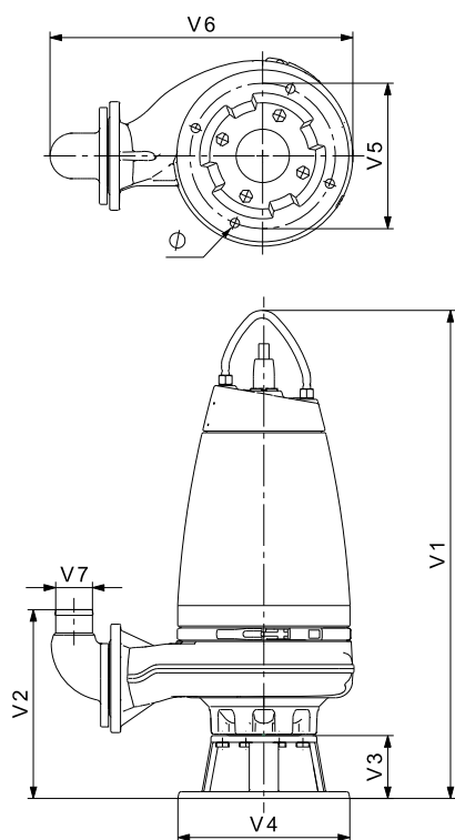
Рис. 5 SE1 Free-standing submerged pump on ring stand
